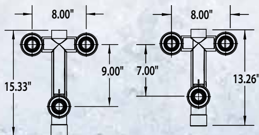
7" Standard Seat Gunitite 3-Jet Manifold
